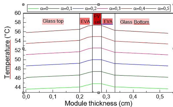
Fig: Temperature profiles within the multilayered structure of a bPV module for various albedo coefficients
