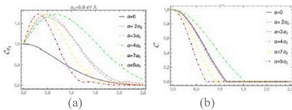
Fig: Dynamical behavior of C11 (a) and C (b) as a function of R for various intensities with \alpha_0 = 0.9 \text{ eV \AA}
