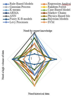
Fig. 2. Parameters related to the reliability of single-model approaches.
