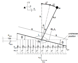
Fig: Flexible structure on elastic-perfectly plastic foundation
