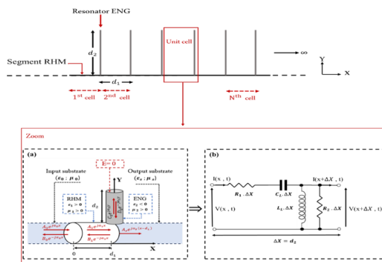
Figure: Schematic representation of a basic unit cell of the transmission line (TL).
