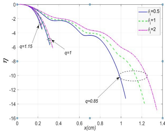
Normalized sheath potential profile for different values of parameter q , and ratio \delta_i = n_{0,Ar^+} / n_{0,He^+}
